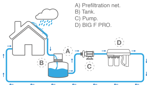
1 RAINWATER TREATMENT
